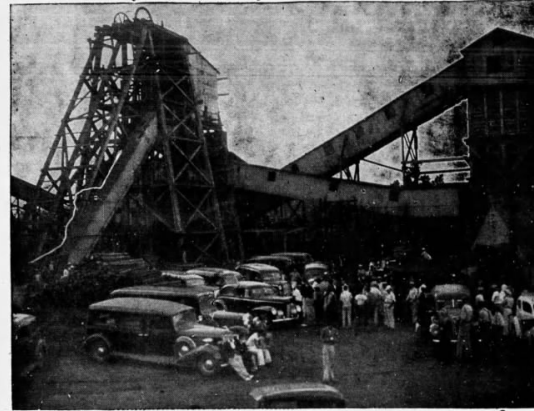
—Evanville Courier-Press Photo The tipple of Duvin mine is shown here. The cars shown here are ambulances kept waiting at the mouth of the mine.
