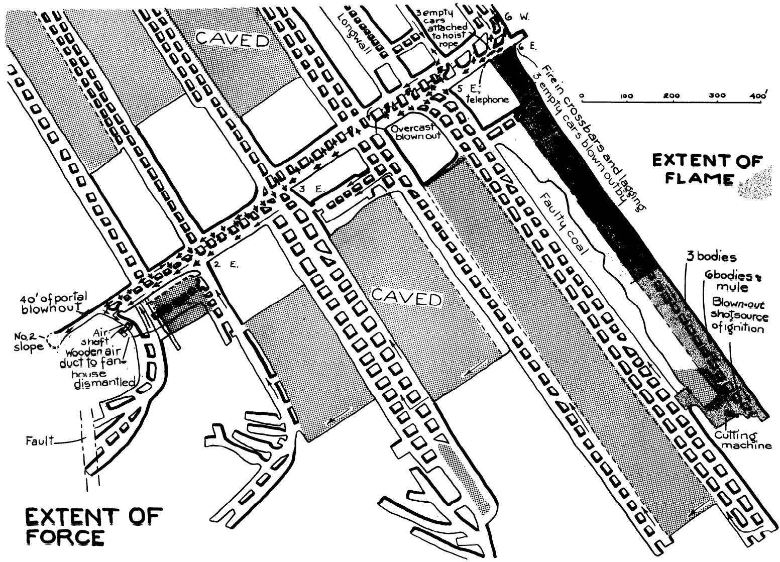
FIGURE 141.—Map of explosion area, Bond Valley mine, Haileyville, Okla., January 17, 1945.
