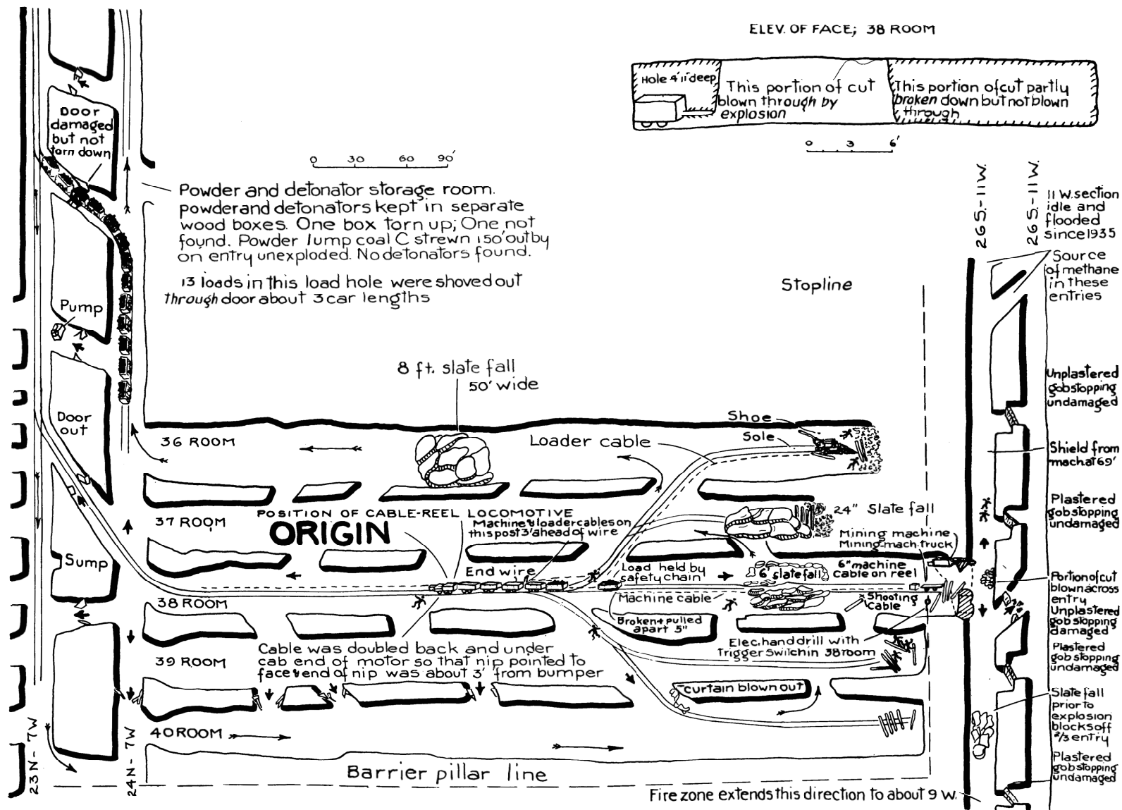
FIGURE 137.—Sketch of explosion area, Nellis No. 3 mine, Nellis, W. Va., November 6, 1943.
