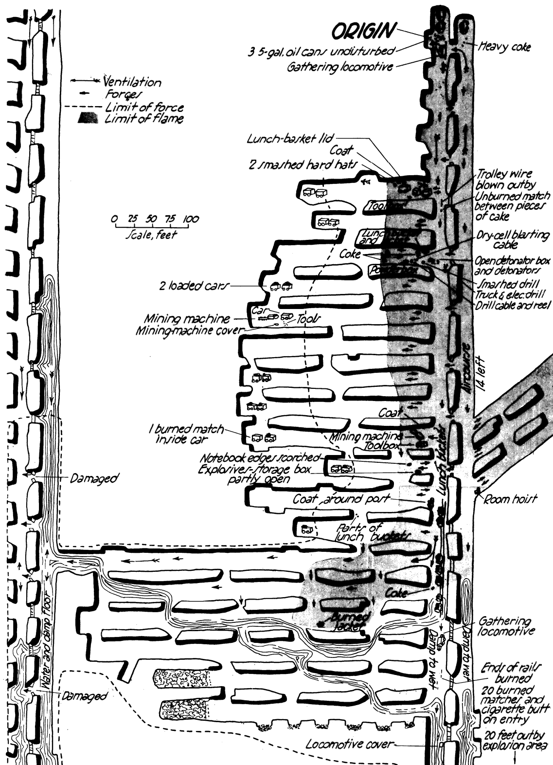
FIGURE 128.—Map of explosion area, West Kentucky No. 10 mine, Wheatcroft, Ky., November 30, 1942.
